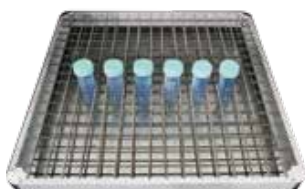
Platform PW-420 W.410 x D.420 x H.65mm (only for ES-60+)
